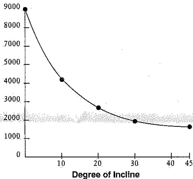
Maximum (Rolling) Weight Capacities on an Incline Weight (Lbs.)
